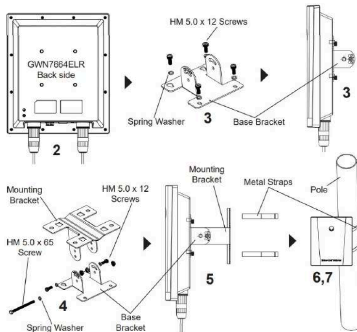
Pole Mount
