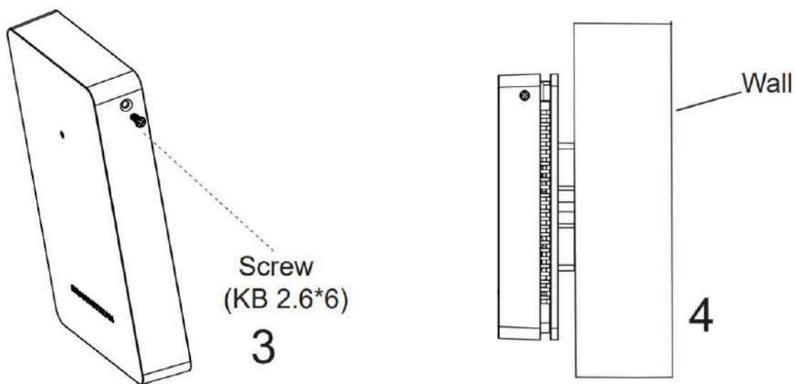
GWN7624/GWN7661/GWN7661E Wall Installation
