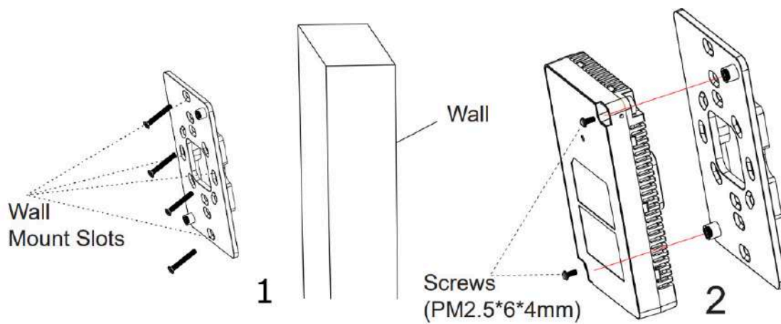
Wall Mount
