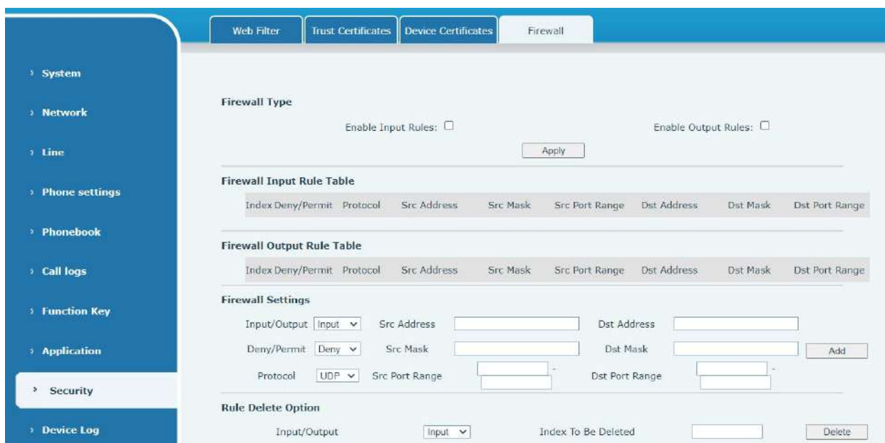
Picture 140 - Network firewall Settings
