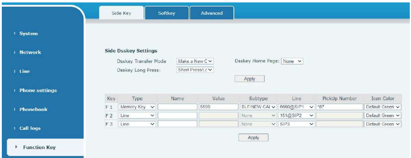
Picture 61 - Web page configuration BLF function key
