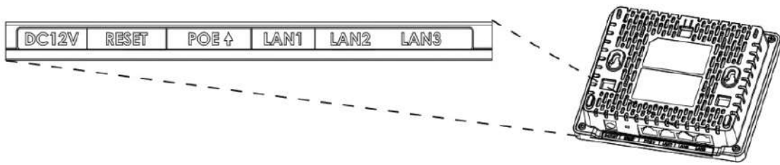
GWN7602/GWN7603 Ports
